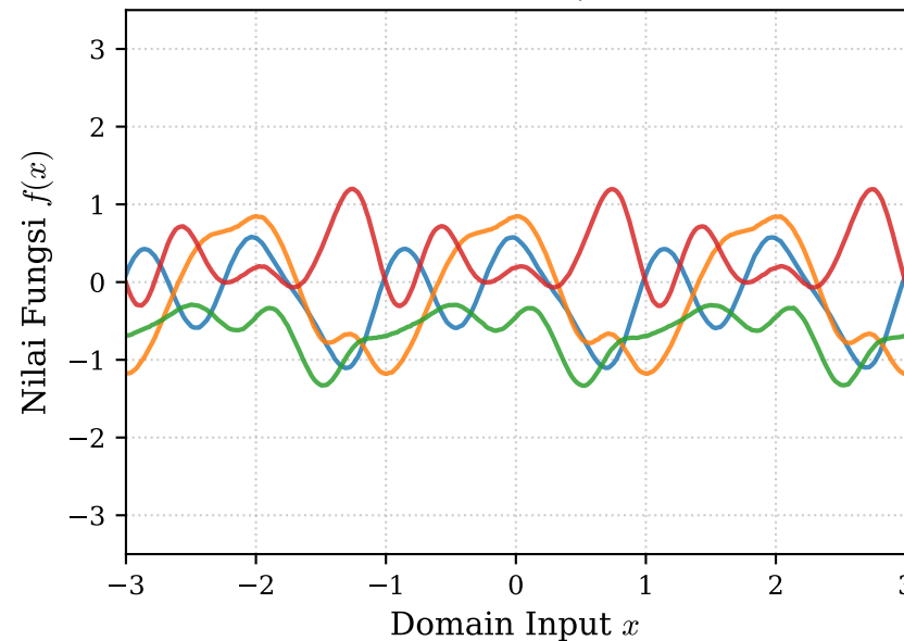
Periodic (Exp-Sine-Squared) ( p = 2.0, l = 1.0, \sigma_f = 1.0 )
