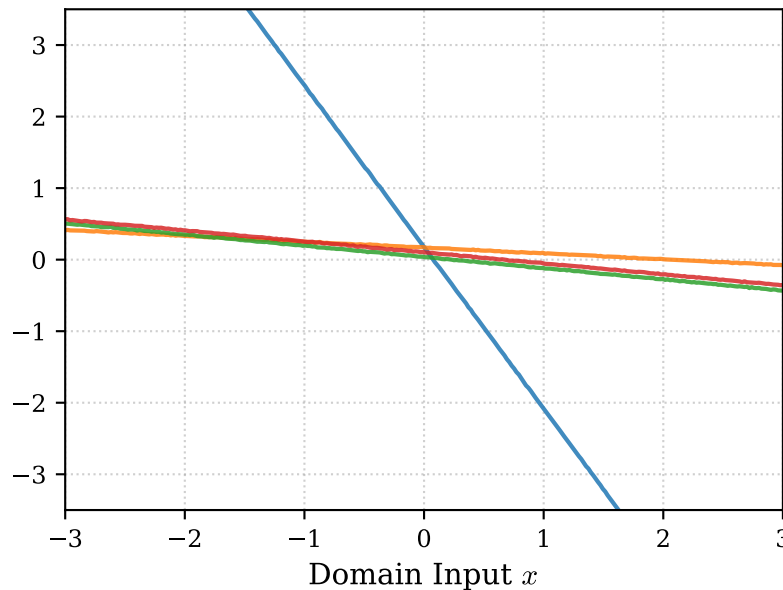
Linear (Non-Stationer) ( c = 0.0, \sigma_b = 0.2, \sigma_v = 1.0 )
