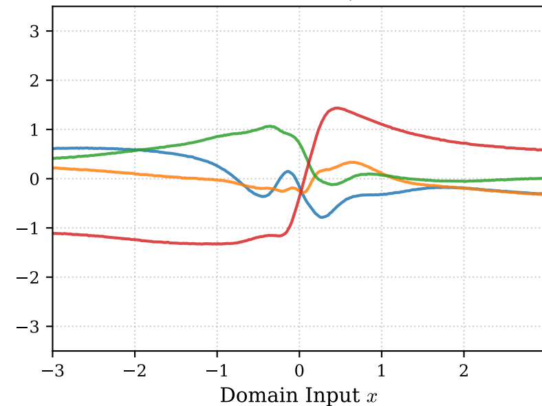
Neural Network (Non-Stationer) ( \sigma_0 = 1.0, \sigma_v = 5.0, \sigma_f = 1.0 )
