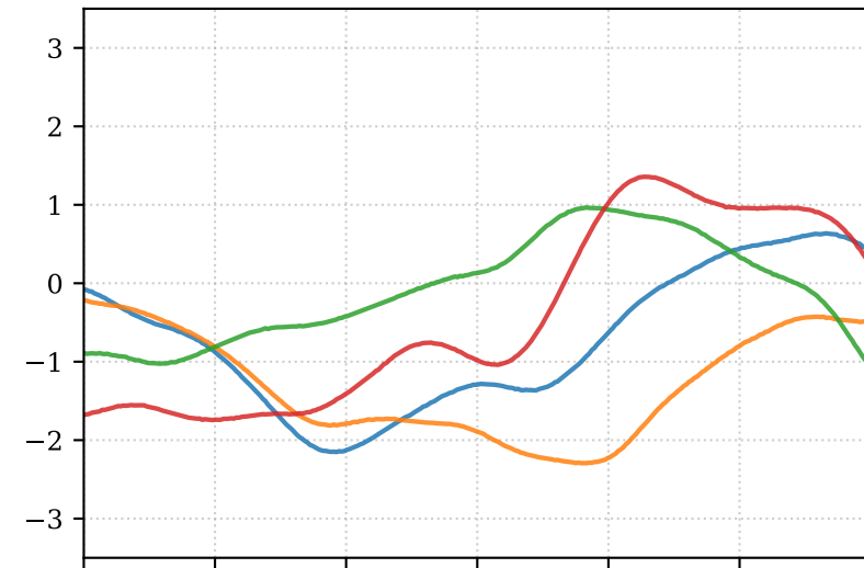
Neural Network (Non-Stationer) ( \sigma_0 = 1.0, \sigma_v = 5.0, \sigma_f = 1.0 )
