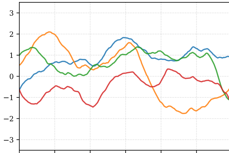
Linear (Non-Stationer) ( c = 0.0, \sigma_b = 0.2, \sigma_v = 1.0 )
