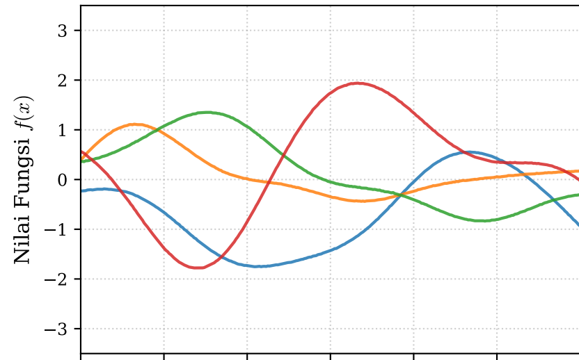
Periodic (Exp-Sine-Squared) ( p = 2.0, l = 1.0, \sigma_f = 1.0 )
